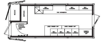
Workshop
