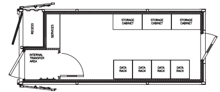
Equipment Cabin
