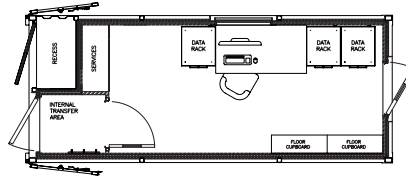
Telecommunications Cabin
